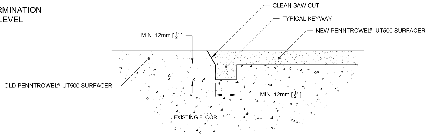
EXISTING PENNTROWEL® UT500 SURFACER TO NEW PENNTROWEL® UT500 SURFACER
