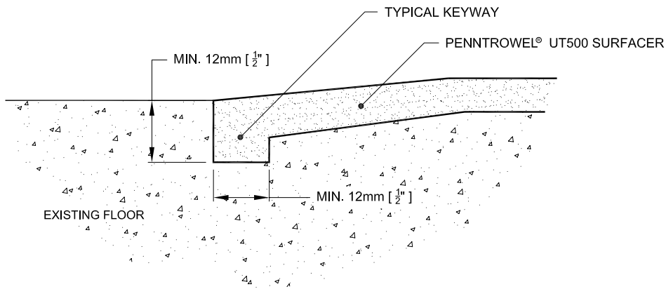
TYPICAL EDGE TERMINATION TO ORIGINAL LEVEL
