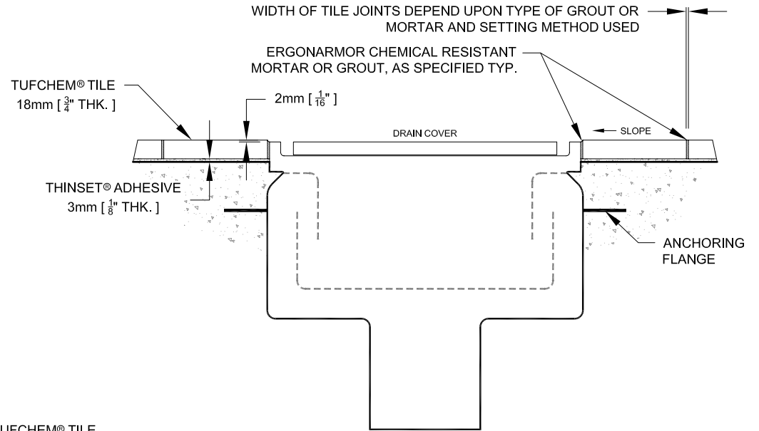
SECTION VIEW
